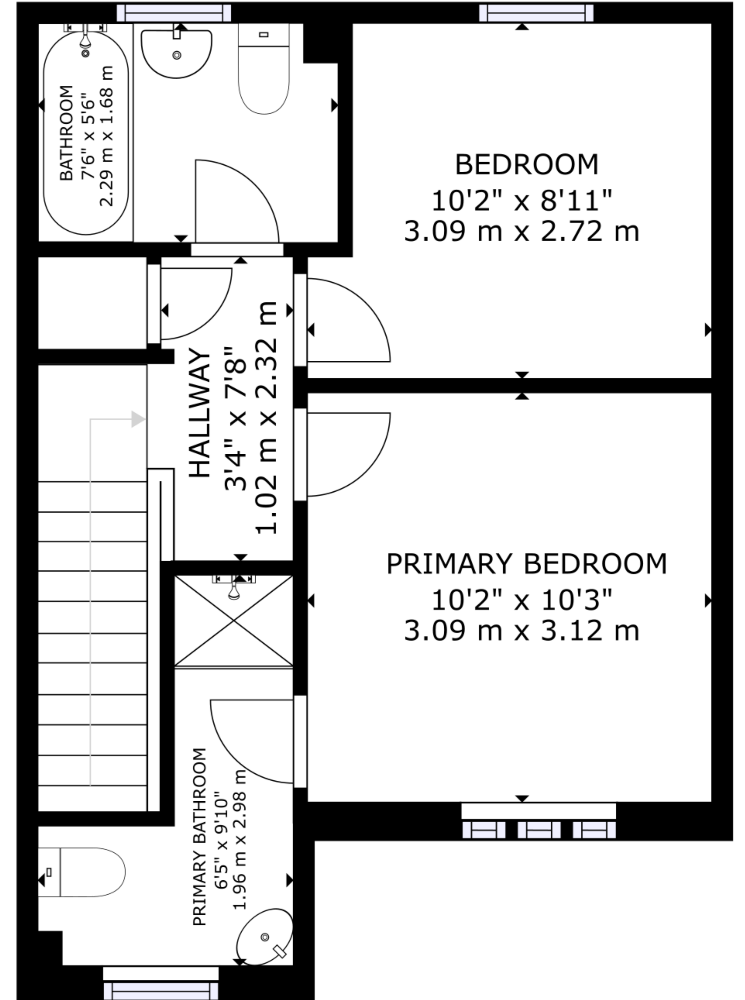
FLOOR 3
